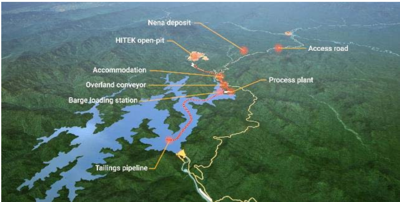
FIGURE 7 - Frieda River Project site layout showing facilities and ISF impoundment area (blue)
